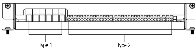
Figure 18 PM235 Terminal
